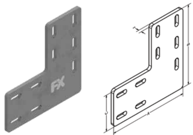
FXT Flat Connector - L
